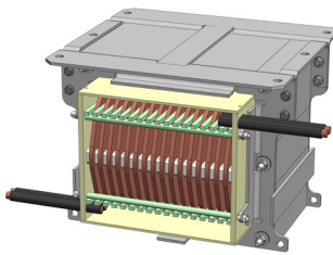
Mantelkerndrossel LFD
